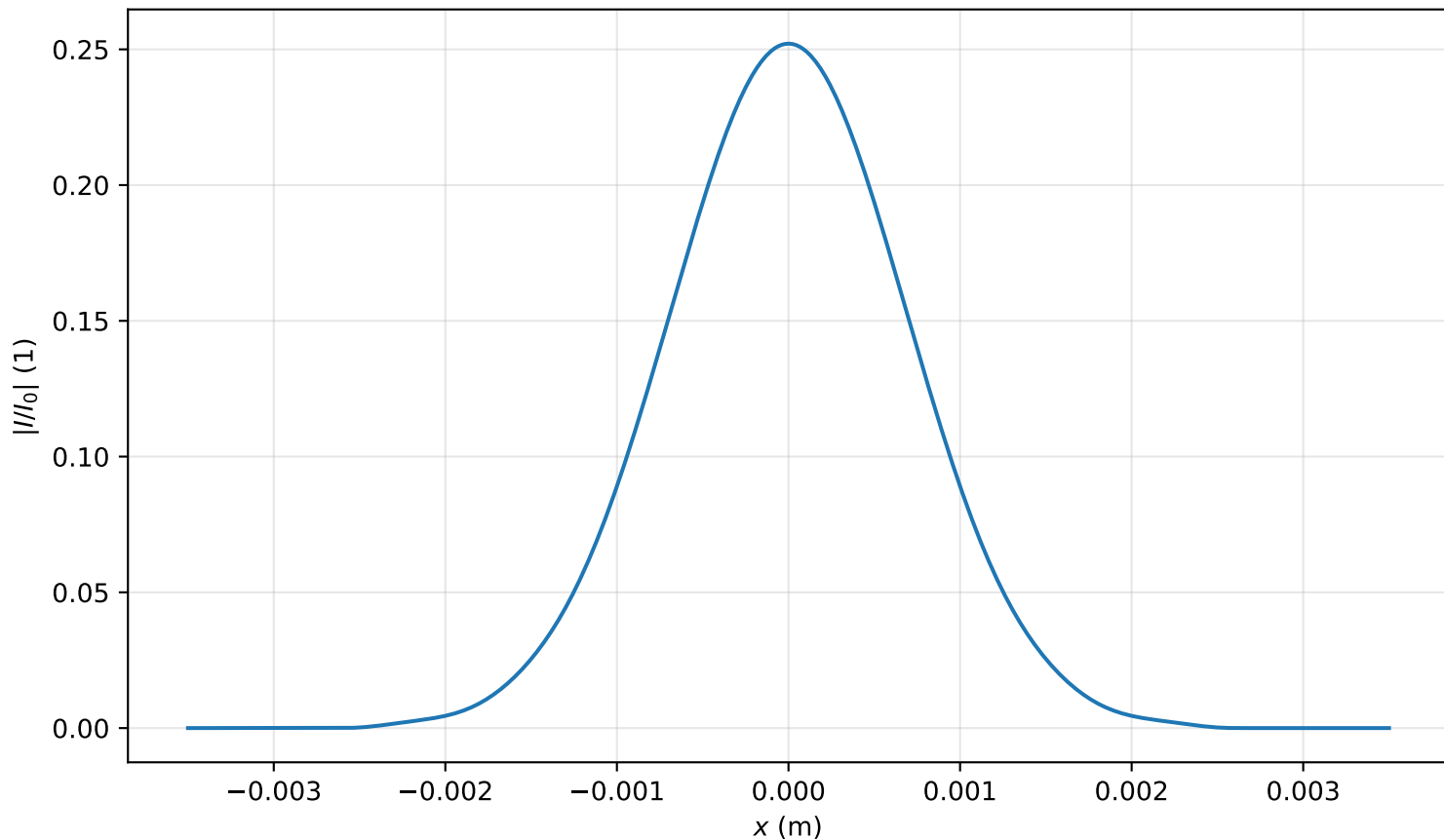
Intensity profile I(x, y = 0, z = 3.662m)/I_0 , P_{in}=0.1P_{cr} , artificial time
